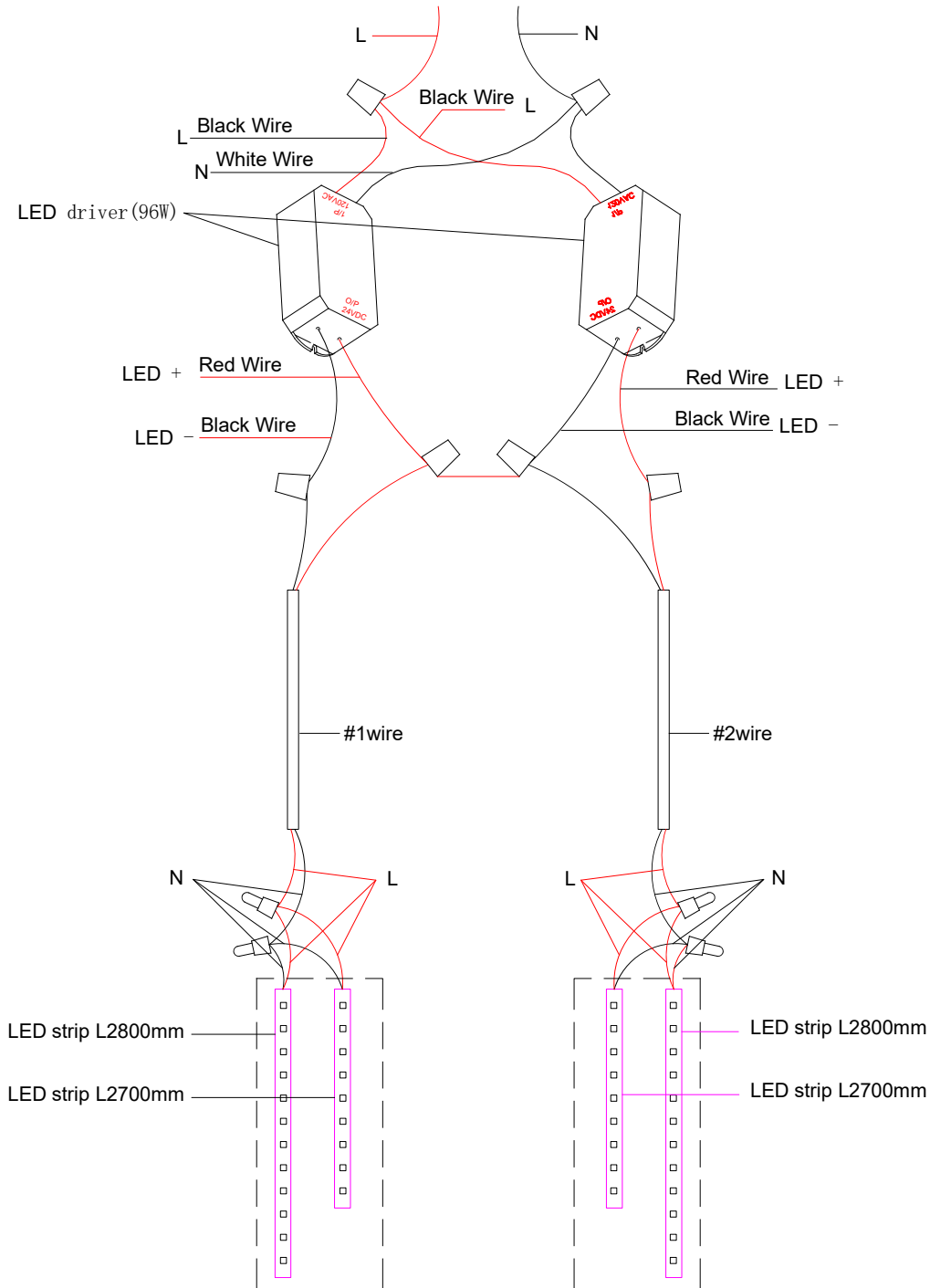
wire diagram
